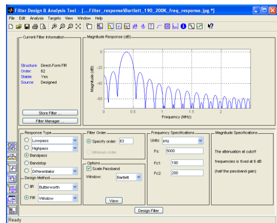
Fig.5. Frequency Response (Bartlett)
