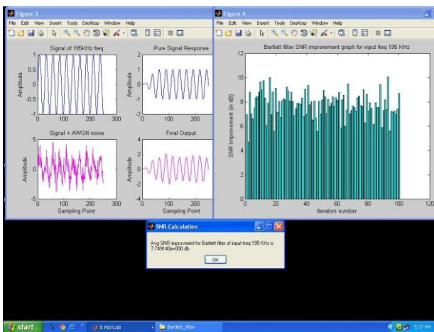
Fig.8. Input signal, signal+ noise, outcomes and SNR improvement (Bartlett)
