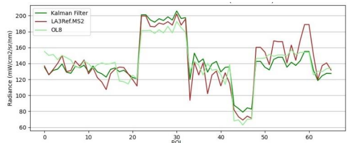
Fig. 23. Validation graph of LA3 radiance with MS2 reference before and after optimization on green channel compared to OL8 radiance.
