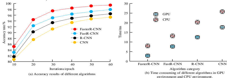
Fig. 11. Performance results of four algorithms.
