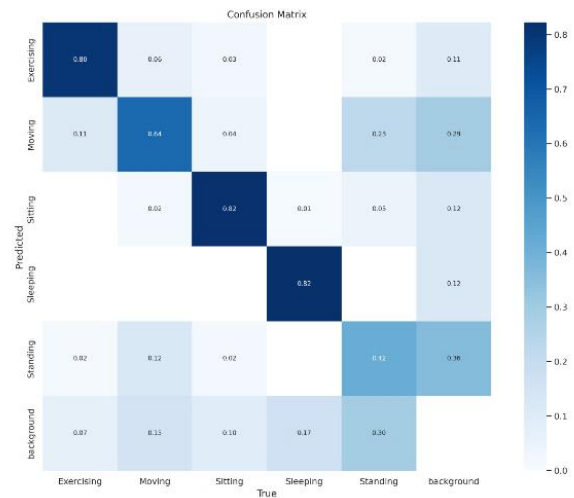
Fig. 12. YOLOv8m model confusion matrix.
