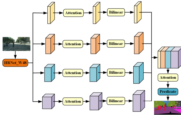
Fig. 5. Schematic diagram of attention mechanism embedding positions.
