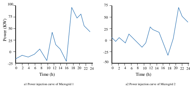
Fig. 7. Upper-level optimization results of Microgrid 1 and Microgrid 2.
