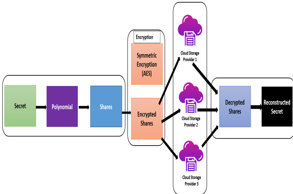
Fig. 1. Proposed model.
