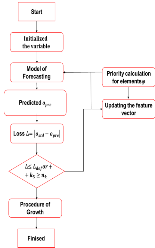
Fig. 1. Adaptive XGBoost.
