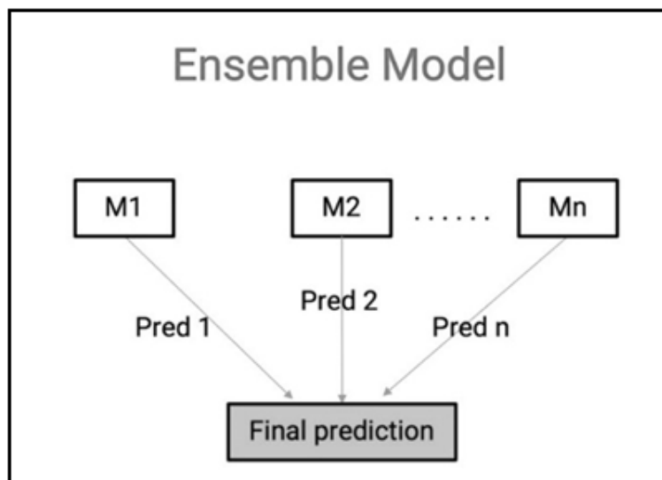
Fig. 3. Ensemble model.
