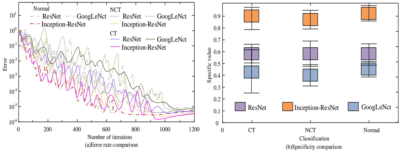
Fig. 7. Comparison of error and specificity.
