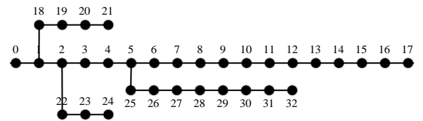
Fig. 4. Schematic diagram of the IEEE 33-bus system structure.
