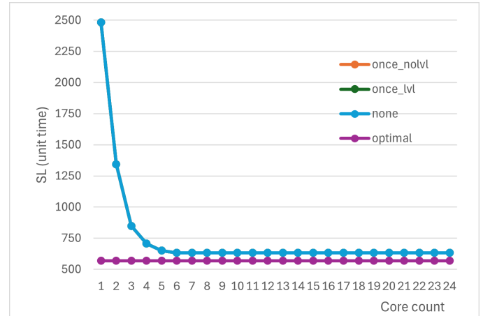
Fig. 10. Scheduling for robot control 88 tasks DAG.
