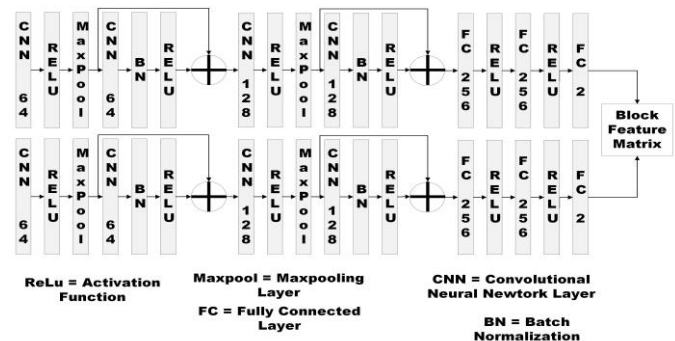
Fig. 2. Siamese neural network architecture.
