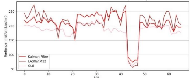
Fig. 22. Validation graph of LA3 radiance with MS2 reference before and after optimization on red channel compared to OL8 radiance.
