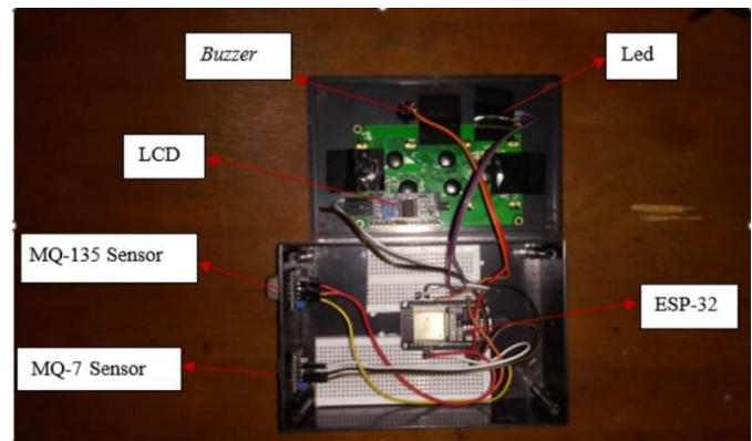
Fig. 3. IAQ hardware implementation.
