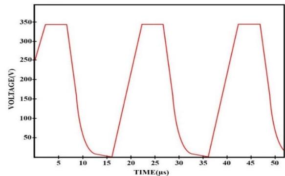
Fig. 9. High voltage generated for Geiger-Müller tube operation.
