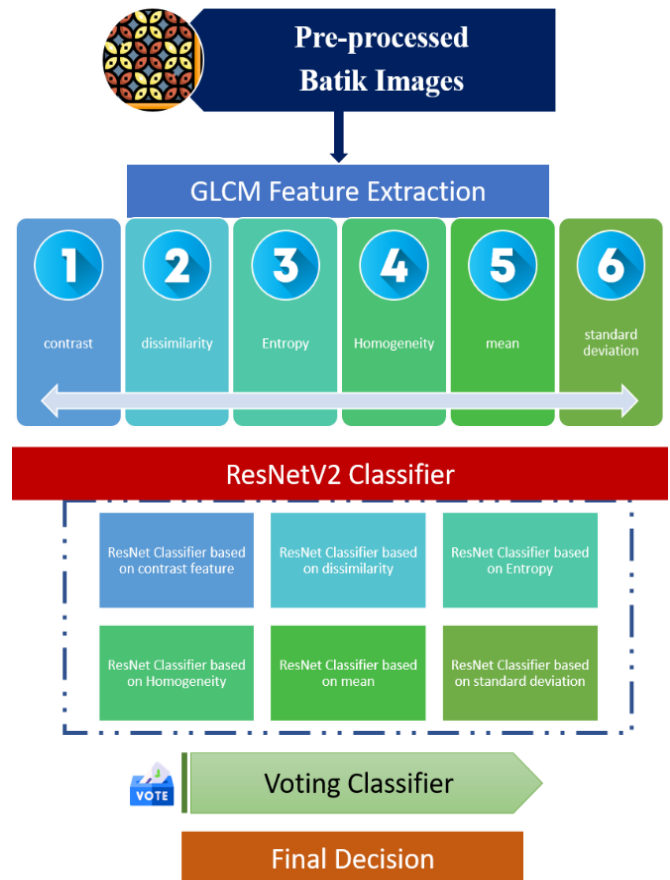
Fig. 4. Flowchart of proposed ensemble deep learning based on GLCM feature extraction.
