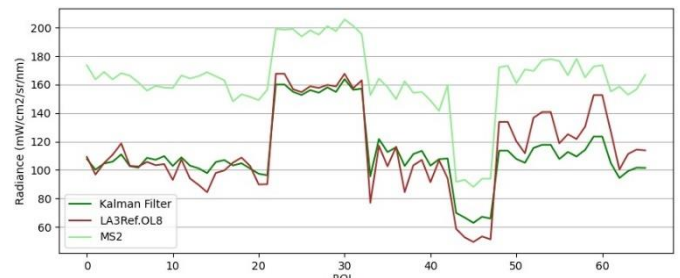
Fig. 19. Validation graph of LA3 radiance with OL8 reference before and after optimization on green channel compared to MS2 radiance.
