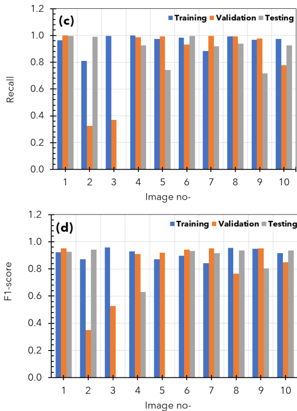
Fig. 8. Performance of sampling image from modified U-Net architecture with freeze in a confusion matrix (a) accuracy, (b) precision, (c) recall and (d) f1-score.
