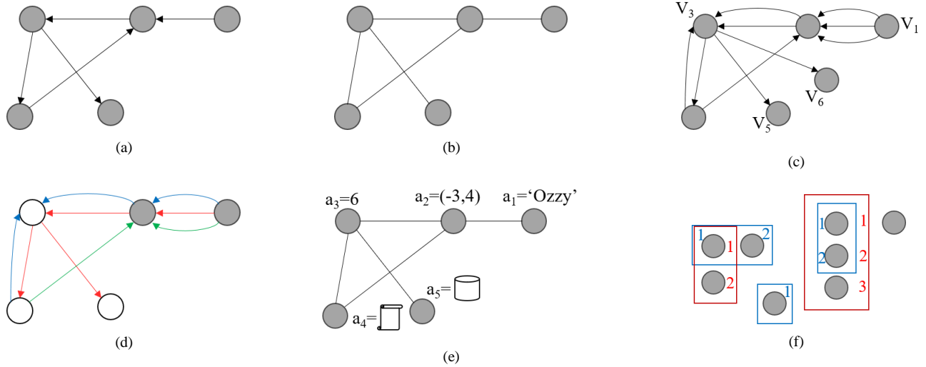
Fig. 2. An overview of different graph types: directed (a), undirected (b), multigraph (c), heterogeneous (d), attributed (e), and directed hypergraph (f).
