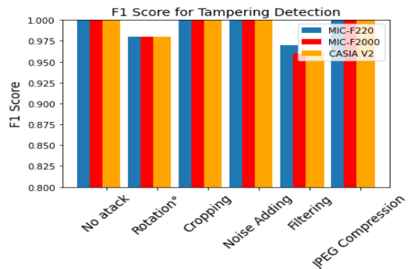
Fig. 10. F1 score for watermark tampering with geometric distortions and image processing distortions.
