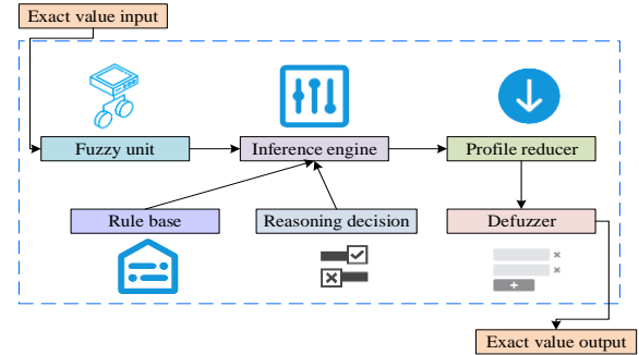
Fig. 4. The structure of RT2FLCM.
