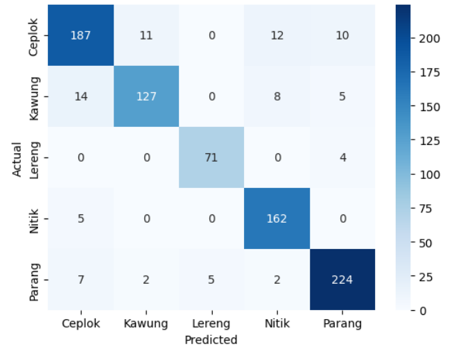
Fig. 9. Confusion matrix based on entropy features.
