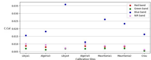
Fig. 6. Average LA3 calibration coefficient with OL8 reference at each calibration site.
