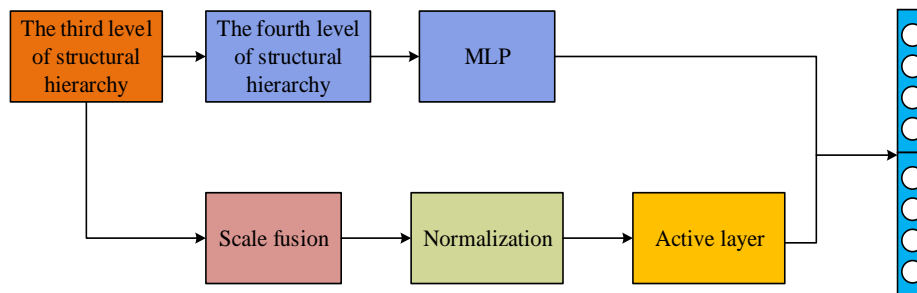
Fig. 5. Feature fusion process.
