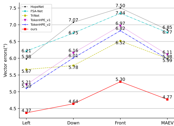
Fig. 8. Comparison with other methods on AFLW-2000 measured by MAEV. Our accuracy exceeds other EAF methods by a wide margin. The lower the better, best viewed in color.
