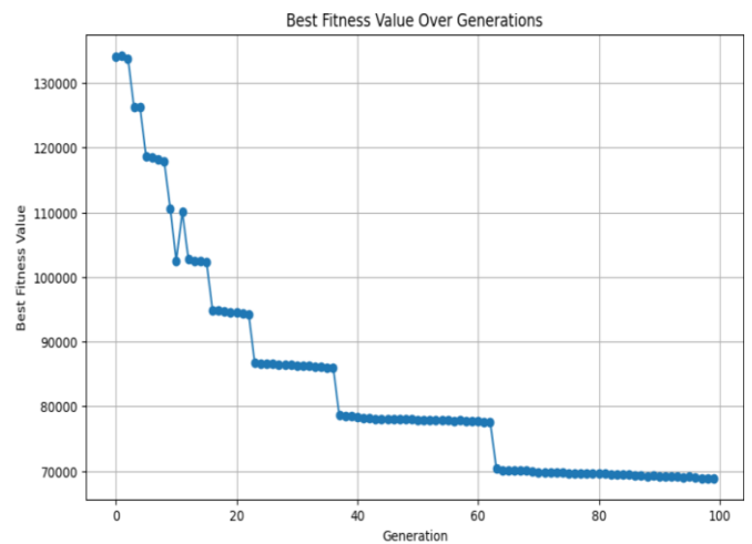
Fig. 6. ACO performance for New York.
