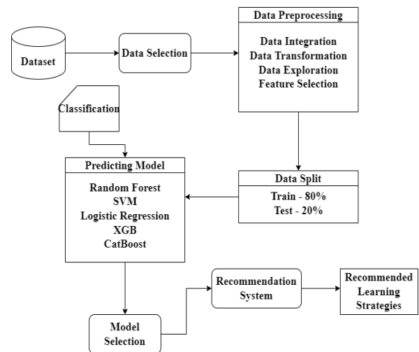
Fig. 2. Research methods for the prediction model.
