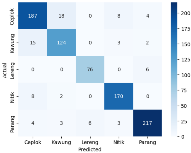
Fig. 8. Confusion matrix based on dissimilarity features.
