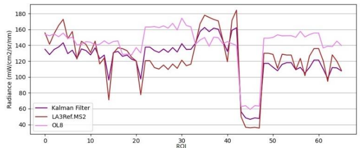
Fig. 25. Validation graph of LA3 radiance with MS2 reference before and after optimization on nir channel compared to OL8 radiance.
