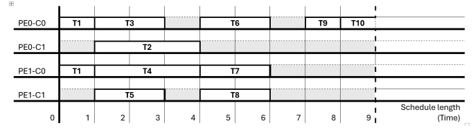
Fig. 6. The schedule generated by CSD algorithm.
