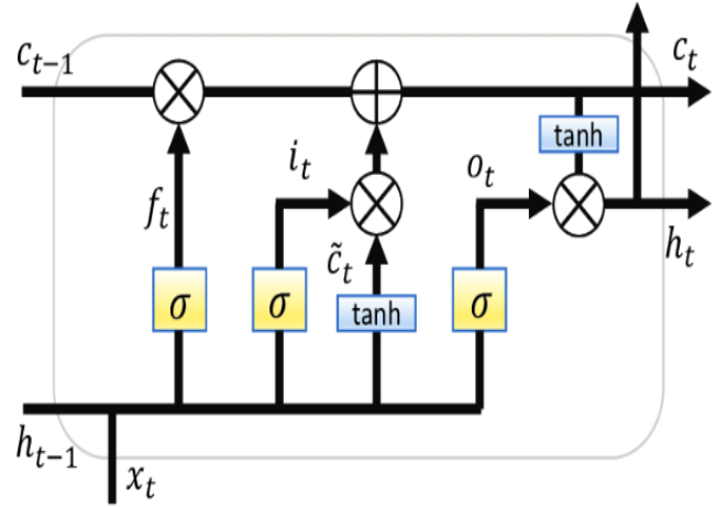
Fig. 2. LSTM architecture.
