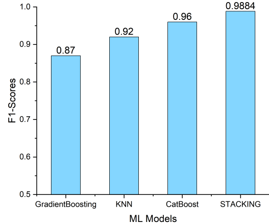
Fig. 3. Metrics of random oversampling.
