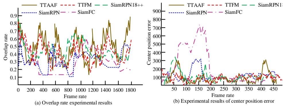
Fig. 10. Comparison analysis curve of overlap rate and center position.
