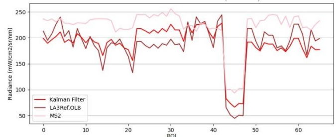
Fig. 18. Validation graph of LA3 radiance with OL8 reference before and after optimization on red channel compared to MS2 radiance.
