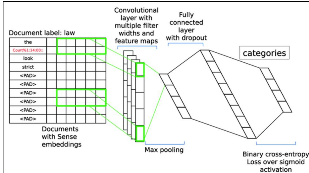
Fig. 2. CNN architecture [23].
