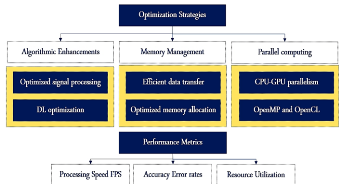
Fig. 10. Optimization strategies.
