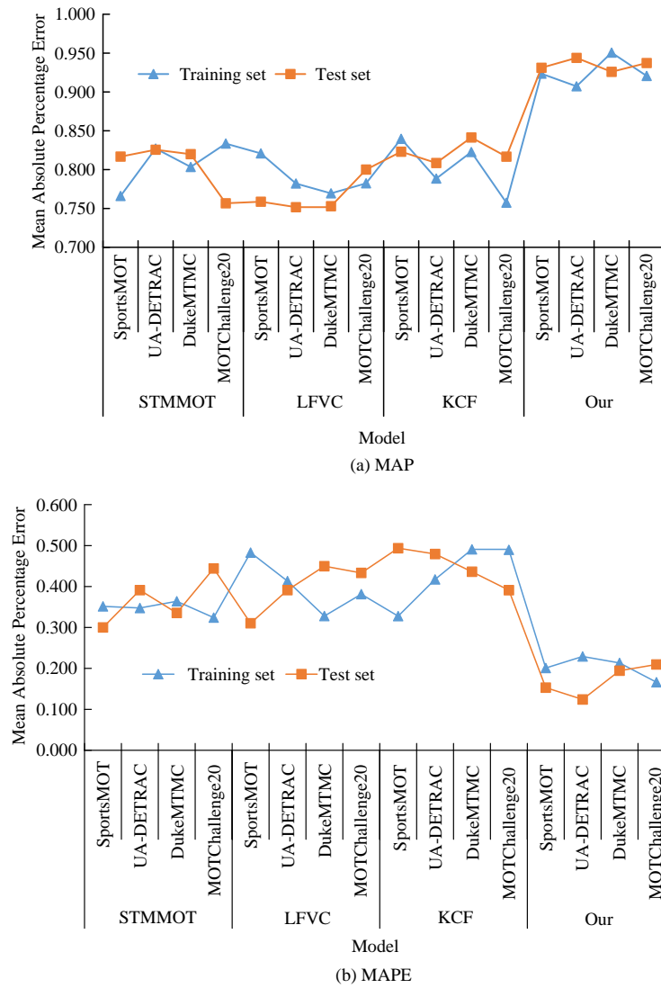
Fig. 9. Comparison of average precision mean and average absolute percentage error for different models.
