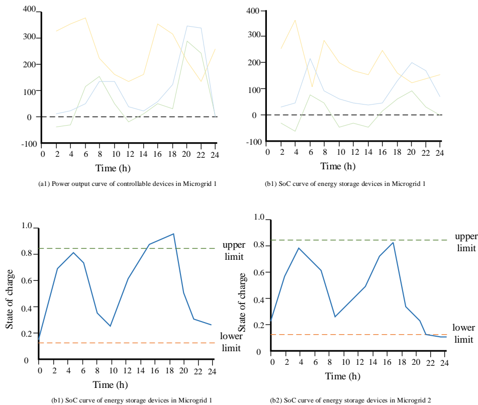
Fig. 6. Lower-level optimization results of Microgrid 1 and Microgrid 2.
