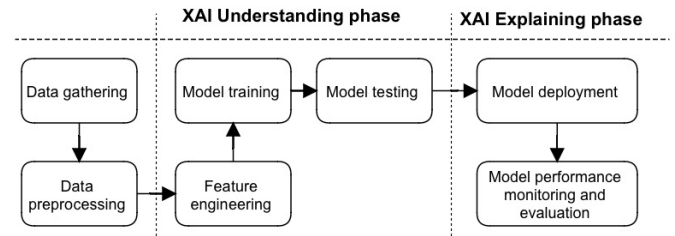
Fig. 1. A typical ML pipeline indicating XAI phases.
