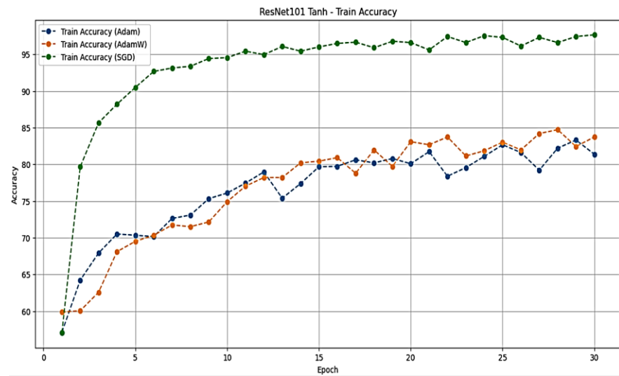
Fig. 4. Comparison of training accuracy using different optimizers.
