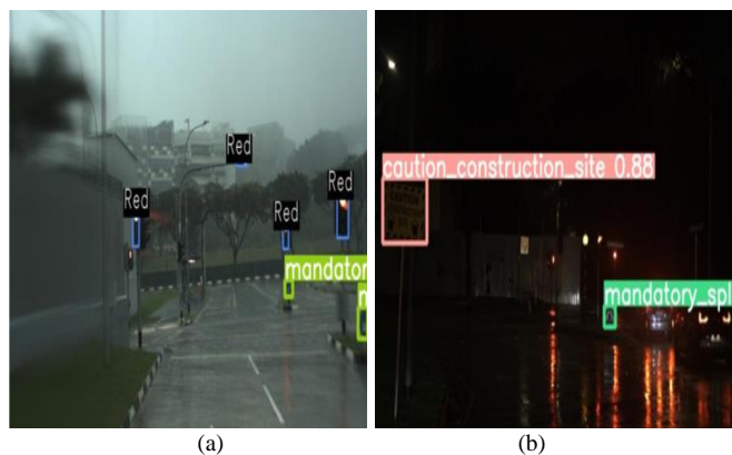
Fig. 5. The image demonstrates the system's detection and recognition capabilities under challenging conditions. (a) Left: the system detects multiple red traffic lights and a 'mandatory left' sign during heavy rain. (b) Right: in low visibility, the system accurately identifies a construction site and split signs but misses a 'give way' sign and a red traffic light (false negatives highlighted in red).
