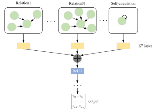
Fig. 6. Schematic diagram of node information aggregation process.
