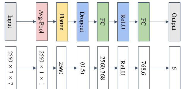
Fig. 4. Upper: MLP architecture with one hidden layer. Lower: the example tensor dimension when use RepVgg_b2g4 as backbone.
