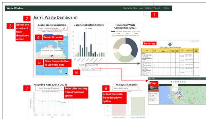
Fig. 13. Dashboard.
