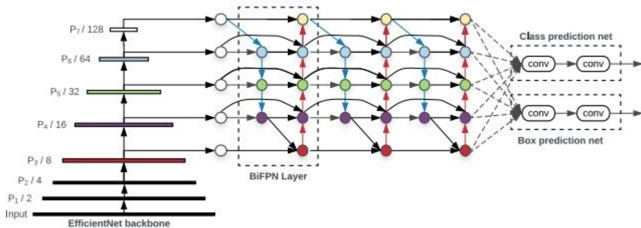
Fig. 2. EfficientDet architecture [31].
