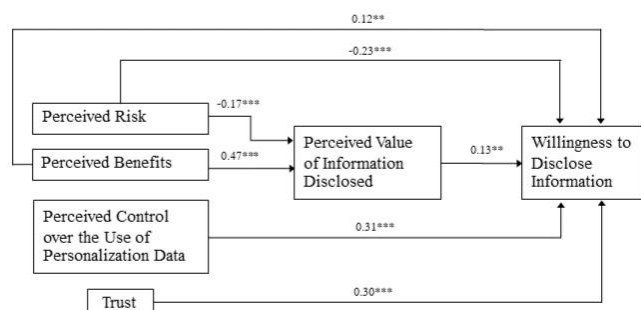
Fig. 3. Adjusted model.
