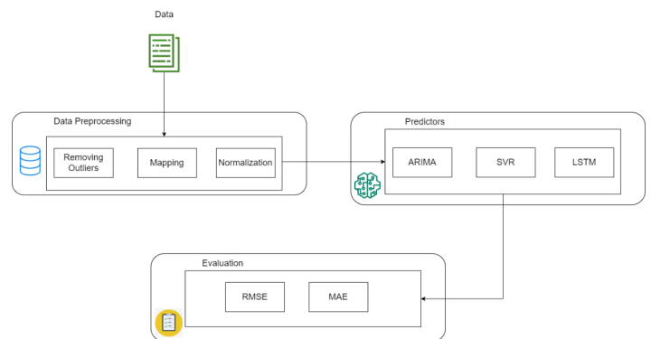
Fig. 1. Workflow process.
