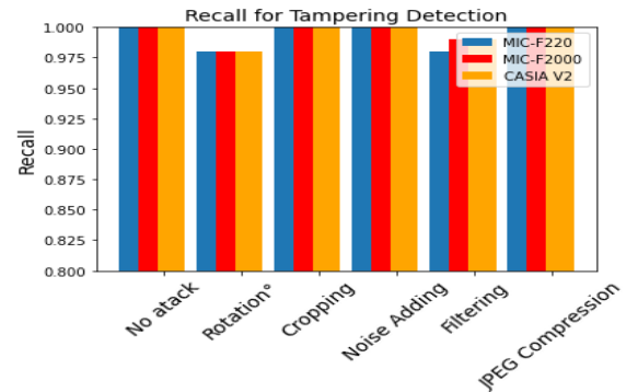
Fig. 9. Recall for for watermark tampering with geometric distortions and image processing distortions.
