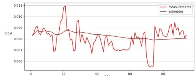
Fig. 10. Calibration coefficients optimization result of LA3 reference OL8 with one-dimensional Kalman filter on red channel.
