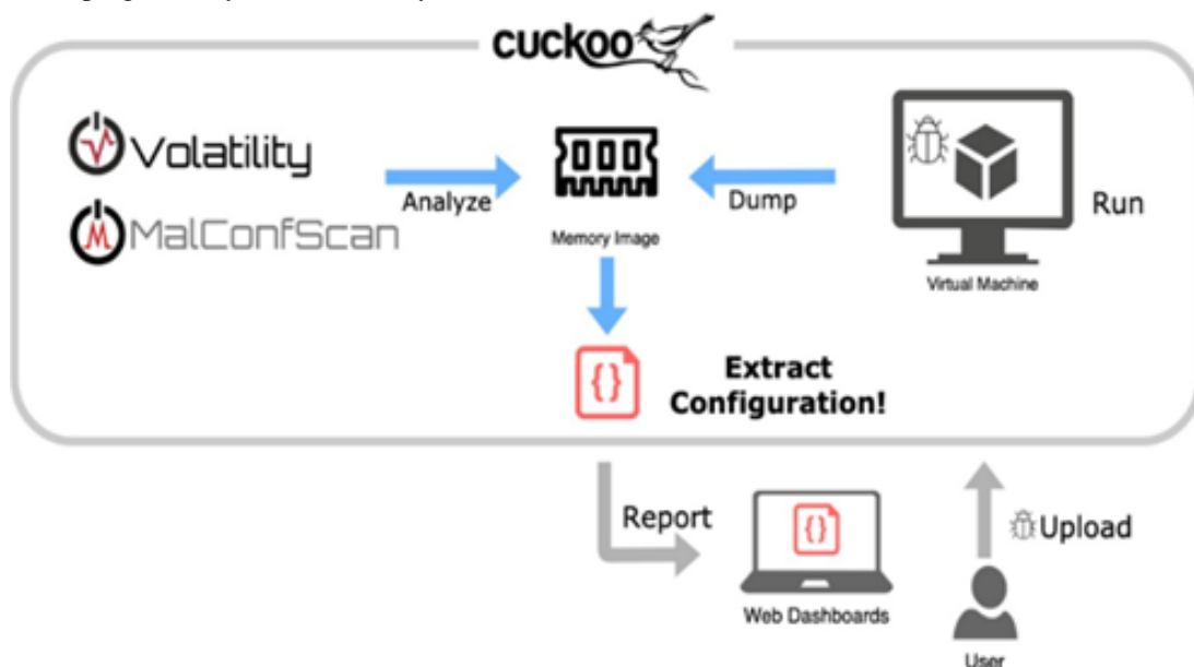
Fig. 18. Non-machine learning detection for ransomware [93].
