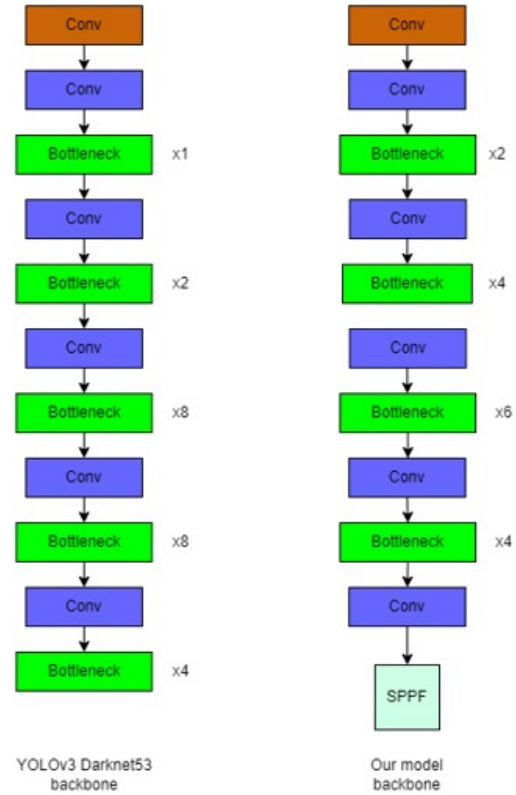
Fig. 2. Backbone of YOLOv3 and our model.
