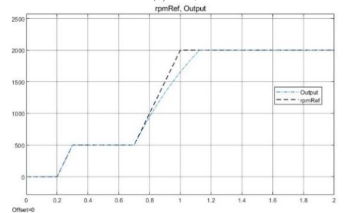
(c) VMF based PID
