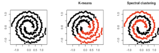
Fig. 3. Difference between K-means and spectral clustering.
