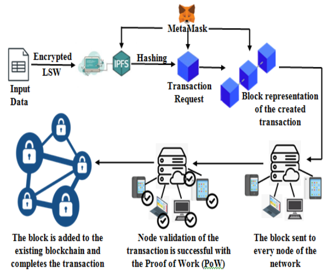
Fig. 2. Blockchain-based data transfer workflow.
