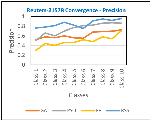
Fig. 5. Reuters-21578 - precision.
