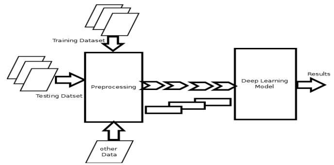
Fig. 4. Solution Process.
