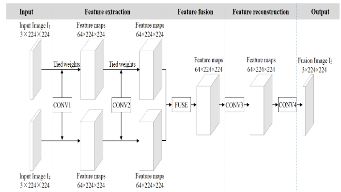
Fig. 3. IFCNN Architecture [14].
