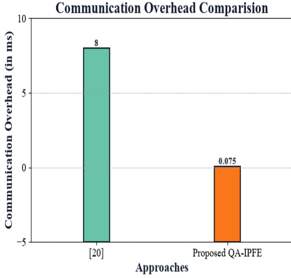
Fig. 4. Communication overhead comparison.
