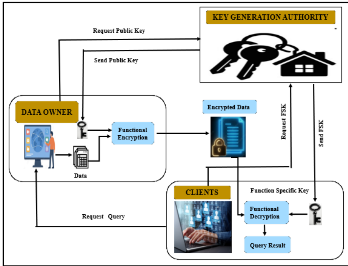
Fig. 1. Proposed architecture of QA-IPFE scheme.
