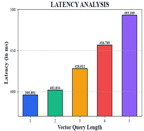
Fig. 6. Scalability of edge processing latency under varying query vector length.
