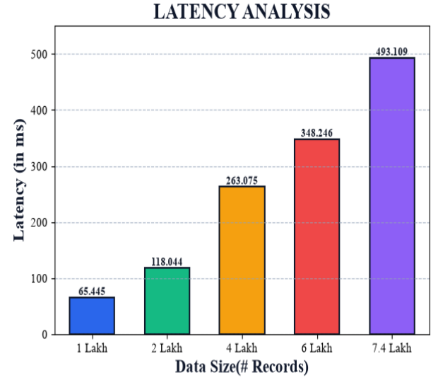
Fig. 5. Scalability of edge processing latency under varying data sizes.
