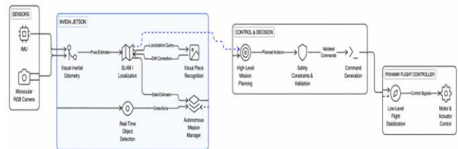
Fig. 3. System architecture.
