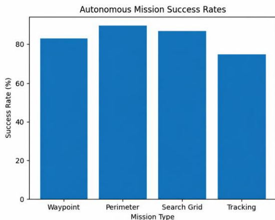
Fig. 5. Autonomous mission success rates in GPS-denied environments.
