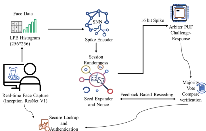
Fig. 2. Architecture of the Face-SNN-PUF system.
