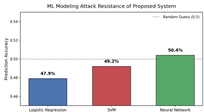
Fig. 7. Prediction performance of machine learning-based modeling attacks (Lower the deviation of random guessing, higher the security).
