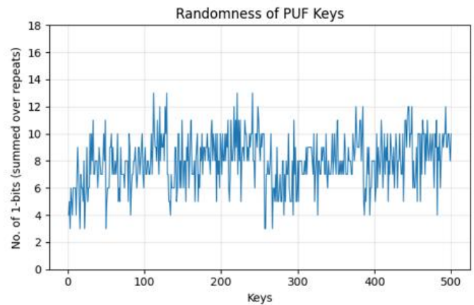
Fig. 3. Randomness analysis of the PUF keys.
