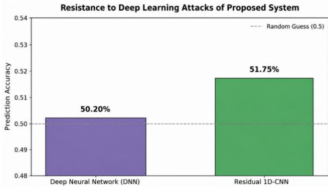
Fig. 8. Prediction performance of deep learning-based modeling attacks (Values close to random guessing indicate higher security).
