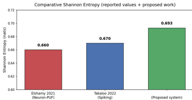
Fig. 6. Comparison of the entropy of the face-SNN-PUF.
