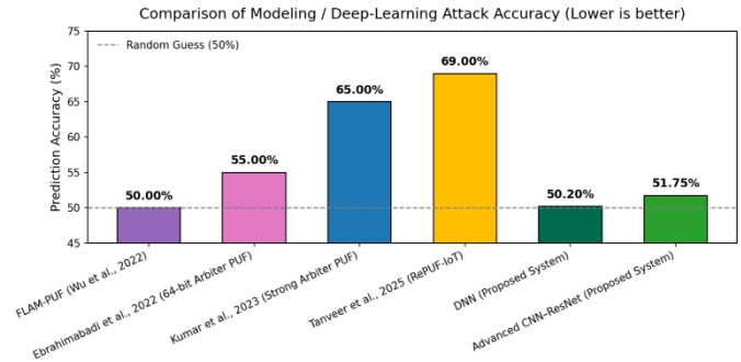
Fig. 9. Comparison of the DL attack resistance of the Face-SNN-PUF.
