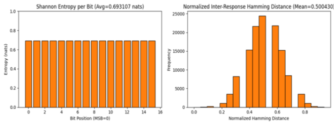
Fig. 5. Entropy and uniqueness of Face-SNN-PUF.
