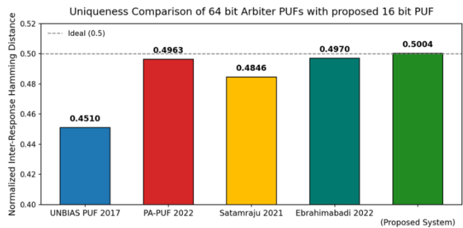
Fig. 4. Comparison of uniqueness of the PUF keys.
