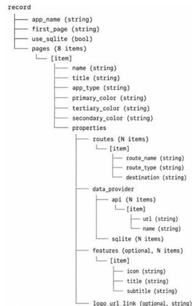
Fig. 1. Structure of the JSON application.
