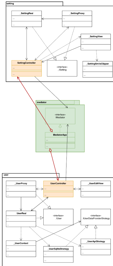
Fig. 3. UML diagram illustrating the mediator pattern implementation.
