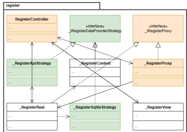
Fig. 4. UML diagram illustrating the strategy pattern implementation.
