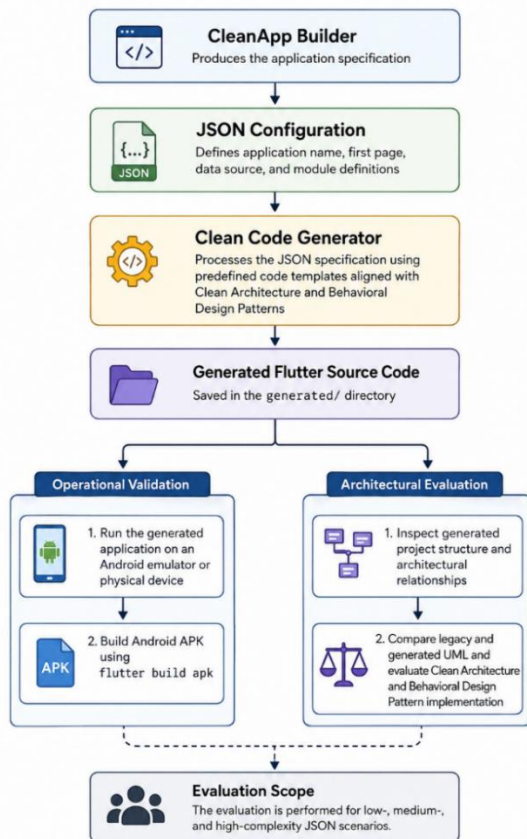
Fig. 2. Workflow of the specification-to-code generation and validation process.
