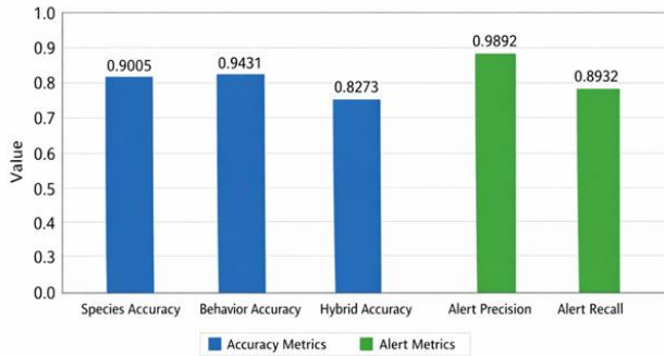
Fig. 18. Performance metrics of the RAID-Net.
