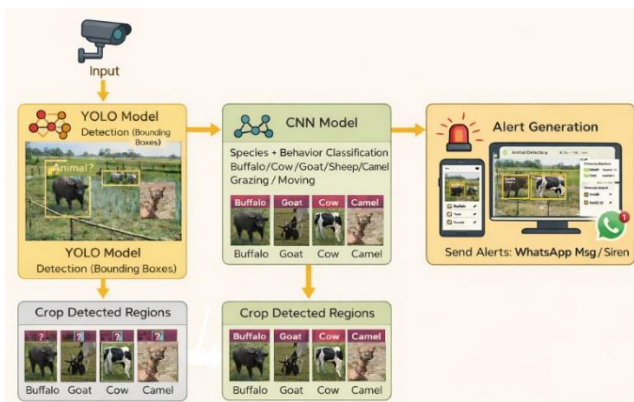
Fig. 10. Architectural framework of RAID-Net.
