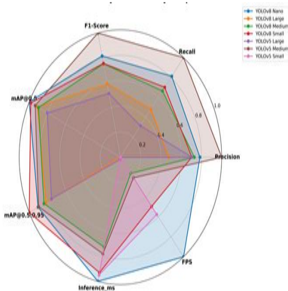
Fig. 14. Holistic performance profiling.
