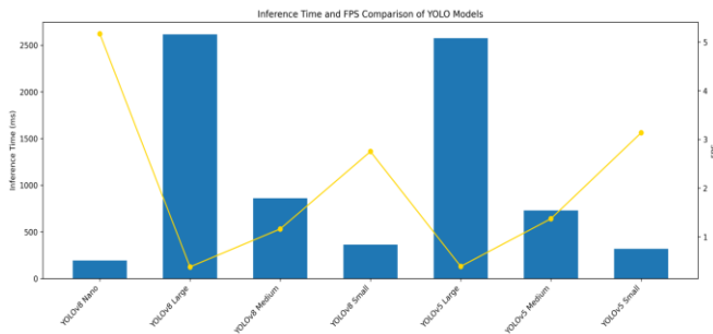
Fig. 13. Computational efficiency and speed.
