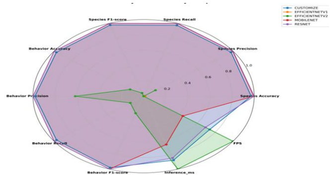
Fig. 17. CNN accuracy and efficiency radar.
