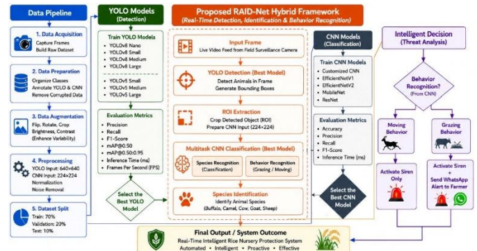
Fig. 3. Flowchart of research methodology and development pipeline.
