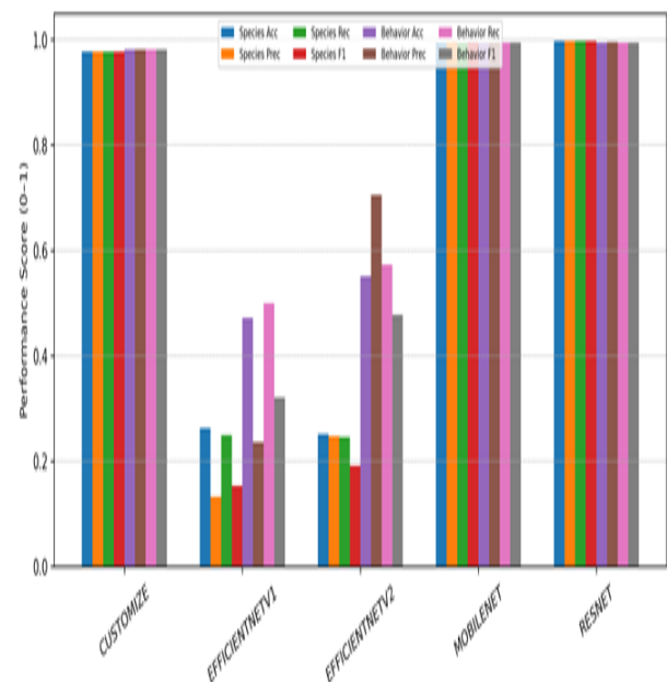
Fig. 15. Classification performance of CNN models.
