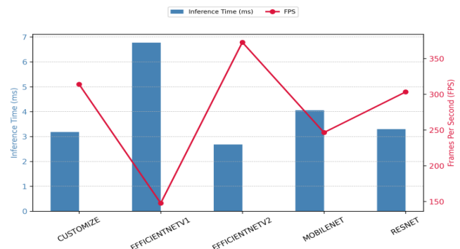
Fig. 16. CNN inference time and FPS.
