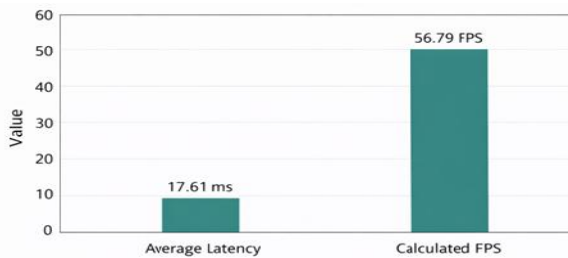
Fig. 19. Latency and FPS performance of the RAID-Net.
