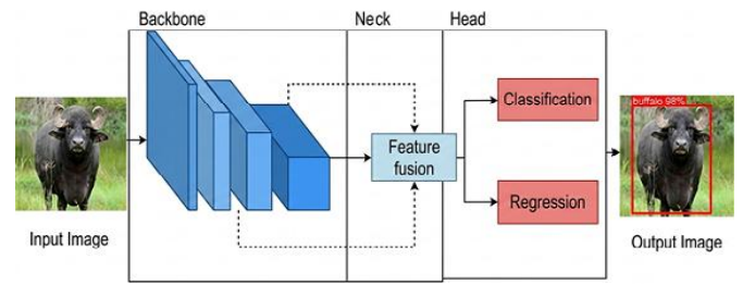
Fig. 8. YOLO architecture.
