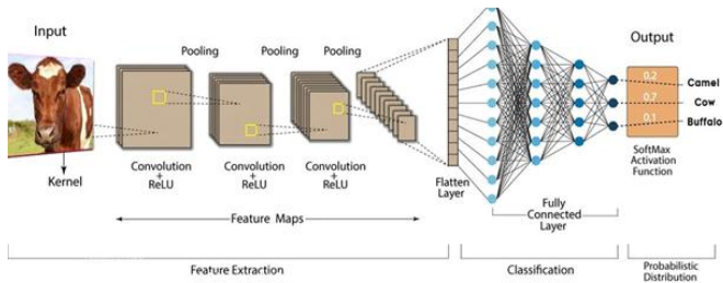
Fig. 9. CNN Architecture.
