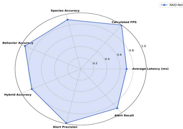
Fig. 20. RAID-Net performance metrics radar chart.
