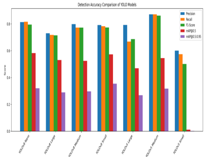
Fig. 12. Detection accuracy comparison.
